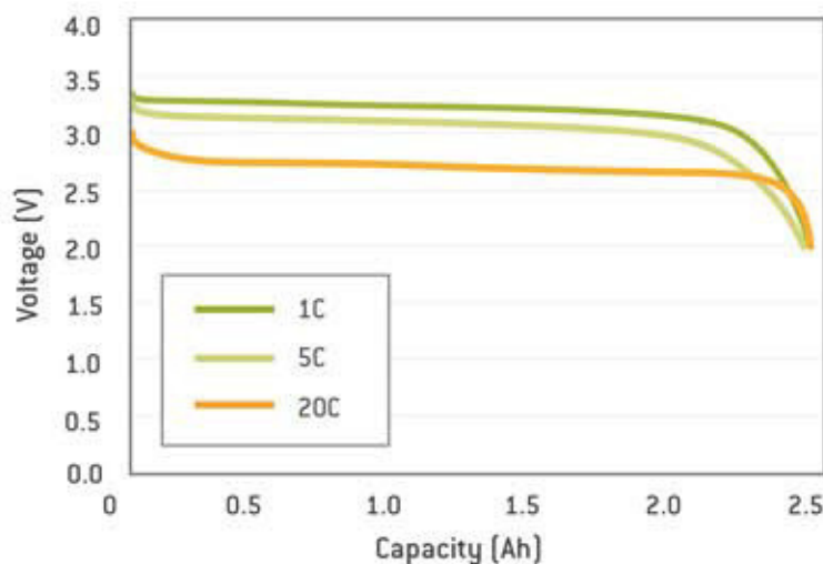
Discharge Characteristics at 23°C
