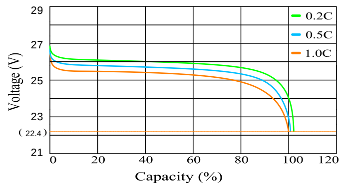
Discharge Performance at 25°C
