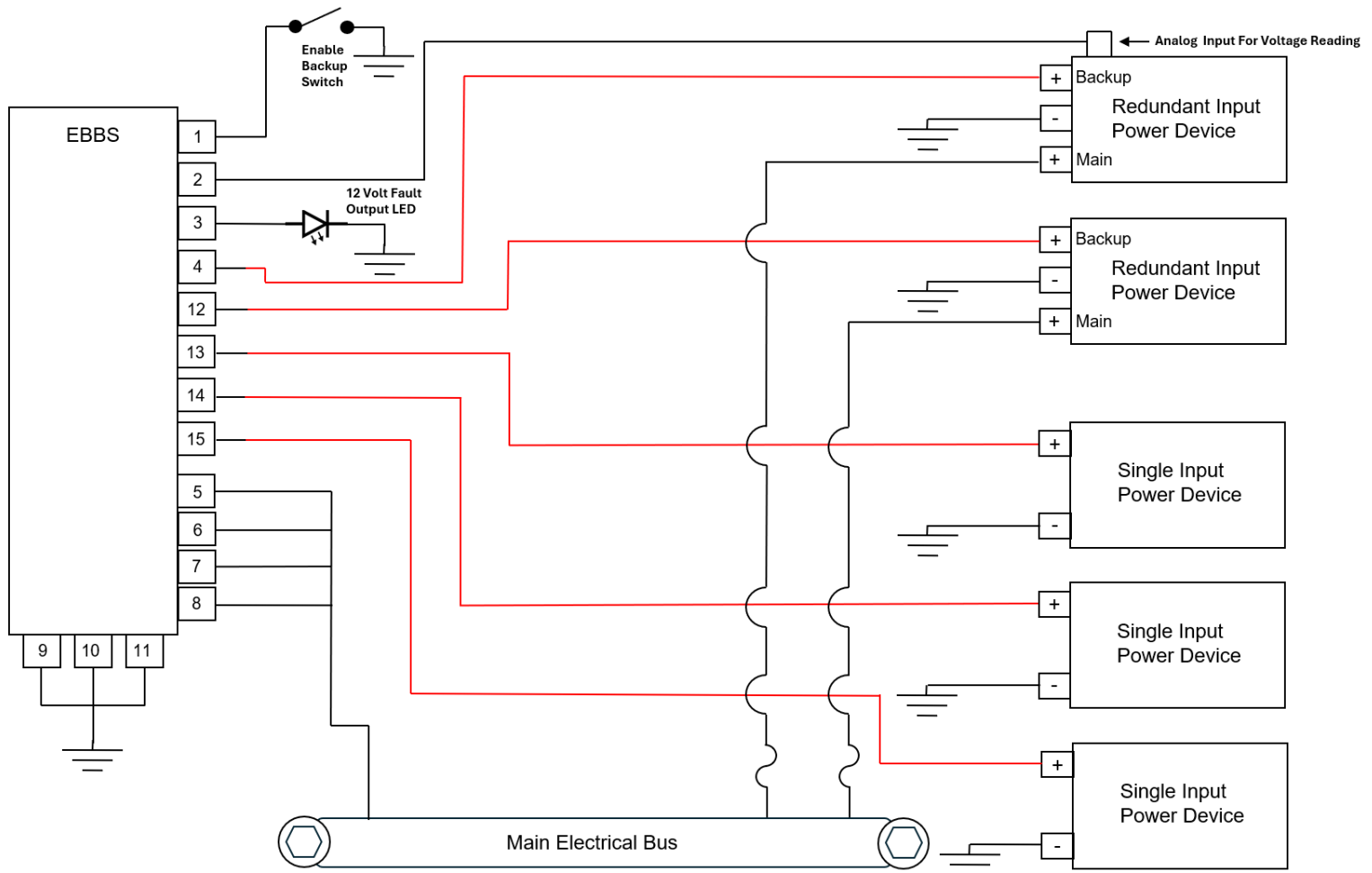
Example Wiring Configuration
