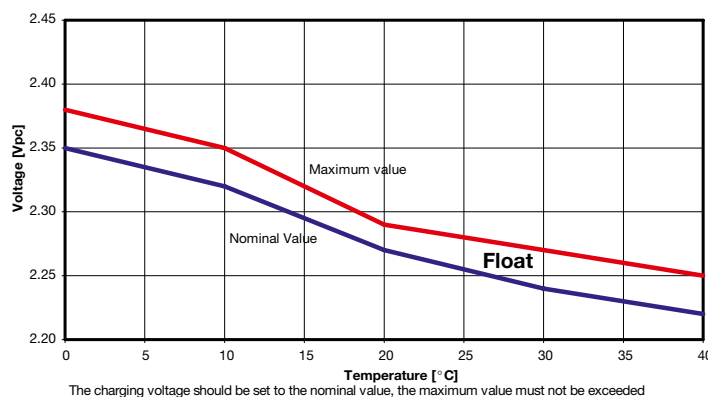
Fig. 1: Marathon L/XL and Powerfit S100/S100L/S300; charging voltage vs. temperature
