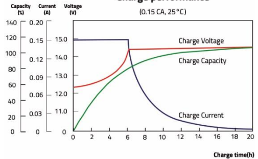
Charge performance
