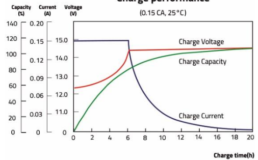
Charge performance
