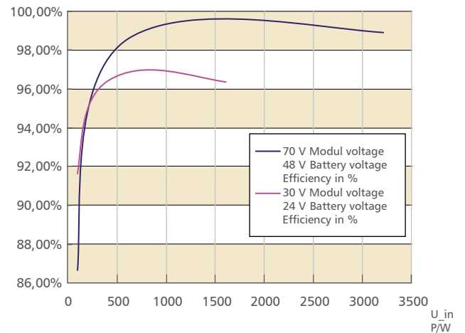
DC-DC efficiency
